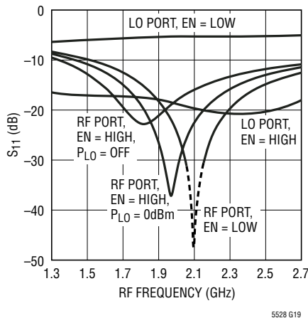
LO and RF Port Return Loss vs RF Frequency
