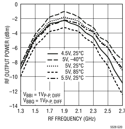
RF Output Power vs RF Frequency at 1Vp-p Differential Baseband Drive
